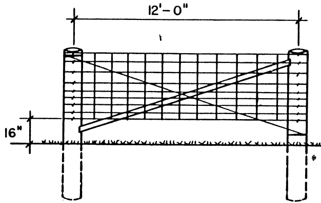
WOVEN WIRE (47 IN., 11-GA.)
