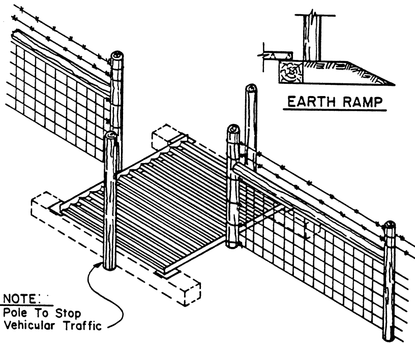
ISOMETRIC VIEW
