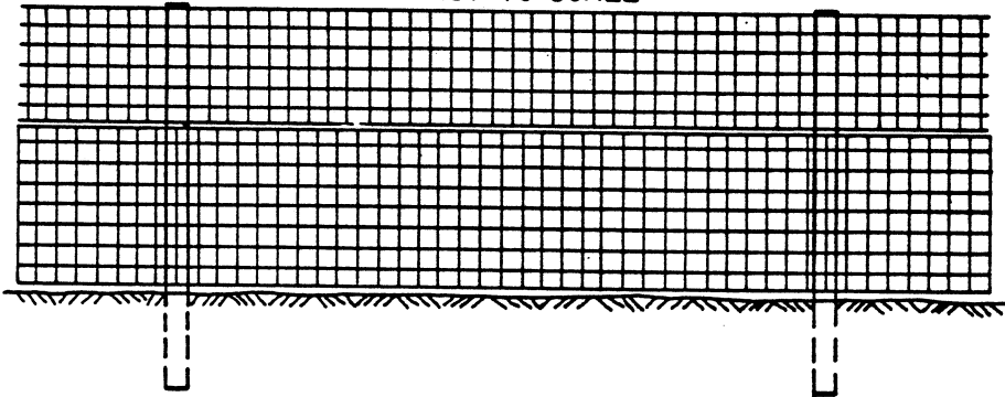
8'-0" HIGH WOVEN/SMOOTH WIRE FENCE NOT TO SCALE
