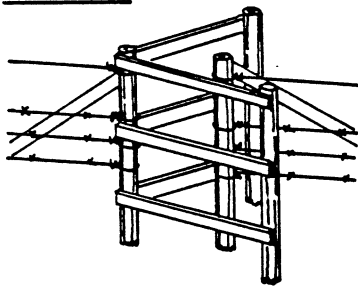
Pedestrian Walk Through
