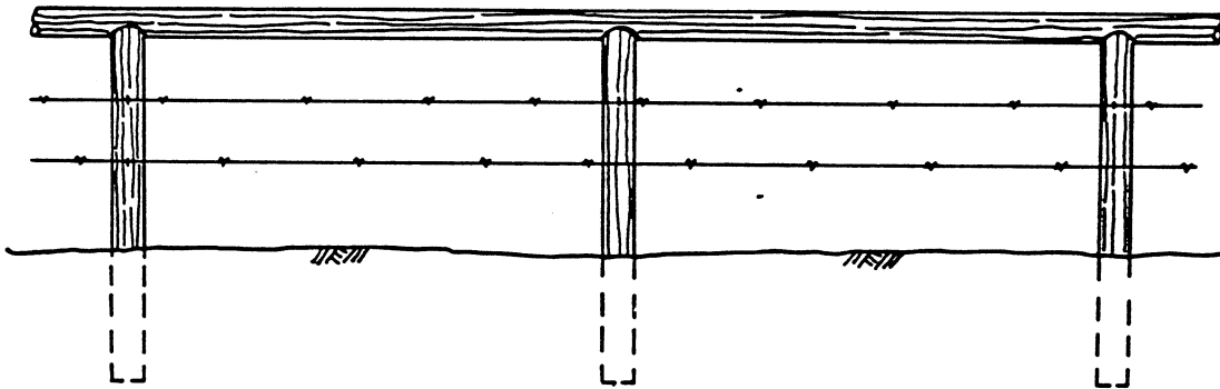
TYPICAL POST, POLE & WIRE FENCE FOR ROCKY MOUNTAIN BIGHORN USE AREAS
