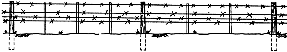
SECTION OF LINE FENCE 4-Wires With 2 Or 3 Stays
