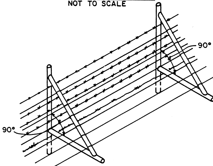
OREGON OUTRIGGER FENCE NOT TO SCALE
