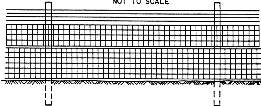
OREGON OUTRIGGER FENCE NOT TO SCALE
