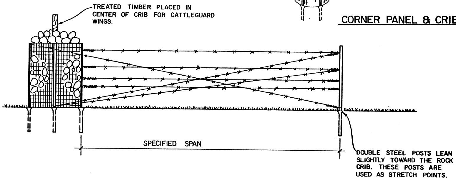
ROCK CRIB & STRESS PANEL NOT TO SCALE
